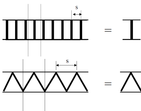
Fig. III 2-12 Extruded Planking
