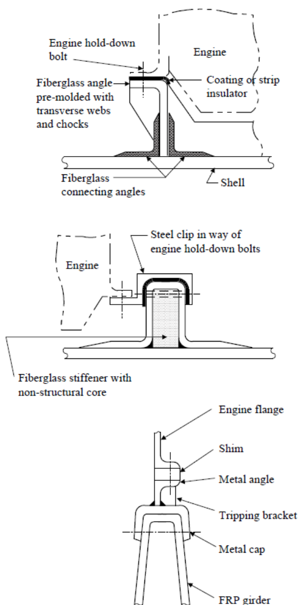
Fig. III 2-25 Engine Foundations
