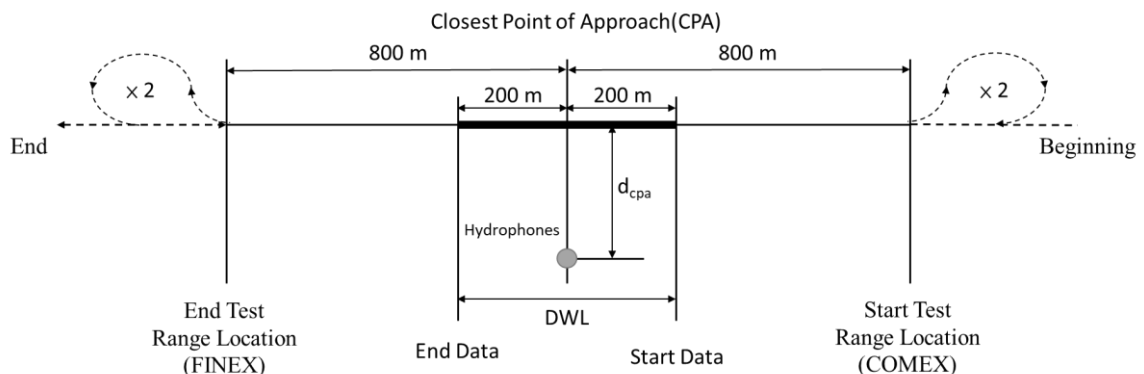
Fig. 3.2 – Ship Operation and Test Range
