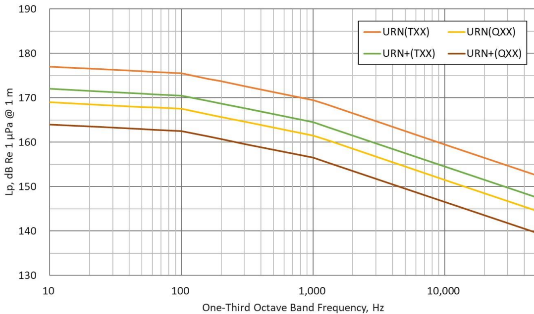
Fig. 3.4 – Acceptance Criteria of Underwater Radiated Noise Level (graph)
