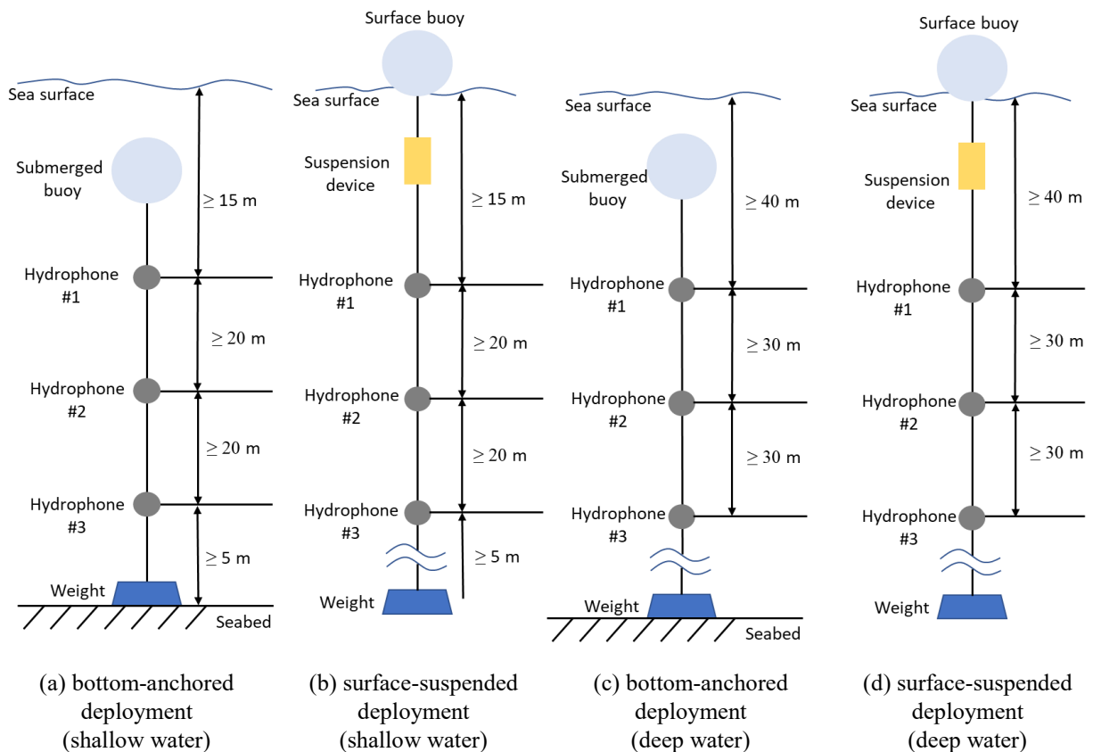
Fig. 3.1 – Deployment of Hydrophones
