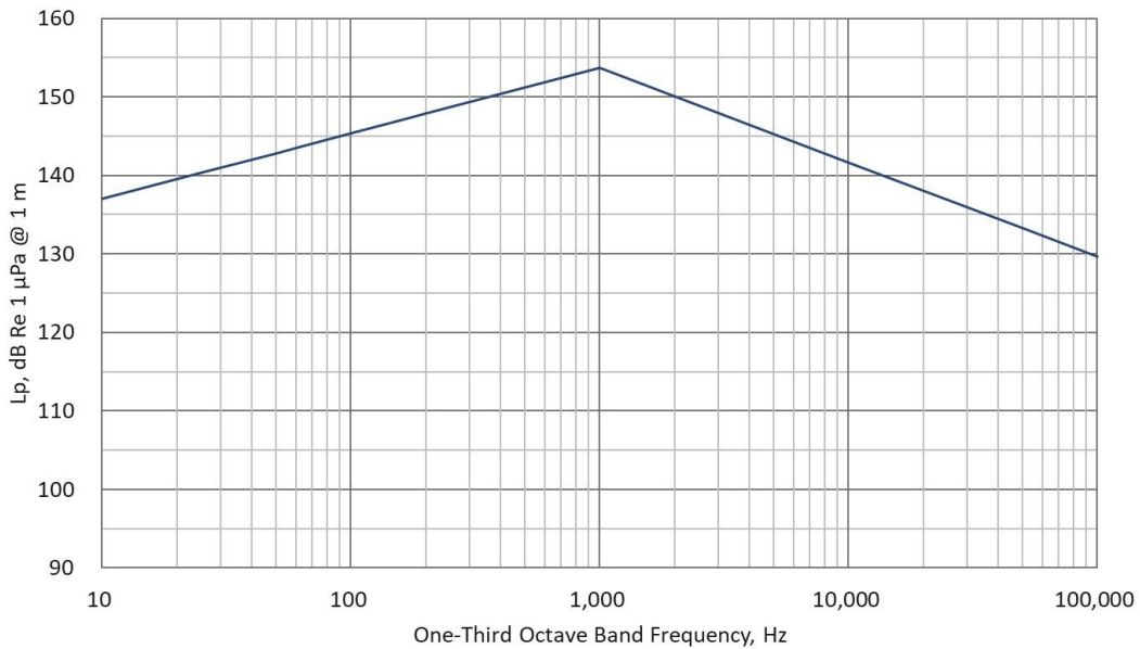
Fig. 3.5 – Allowable URN Limits for Research Vessels
