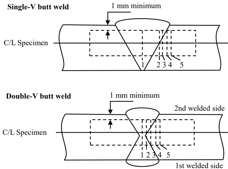
Figure 6.2 – Orientation of Weld Test Specimen
