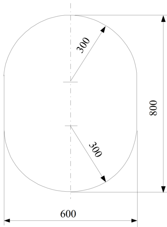
CR Fig. 3-1 Vertical Openings
