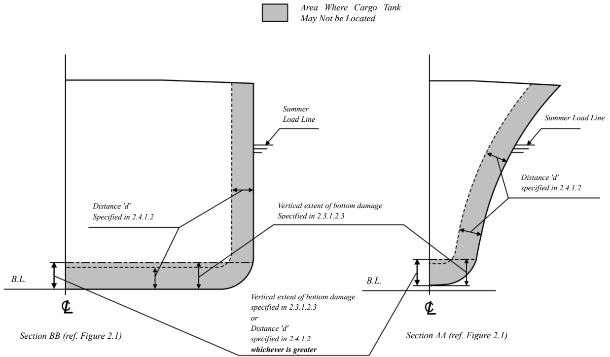
Transverse Sections – Type 2G and 2PG Ships
