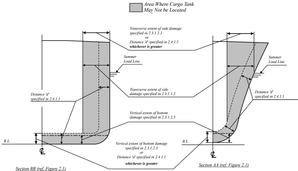
Transverse Sections - Type 1G Ship
