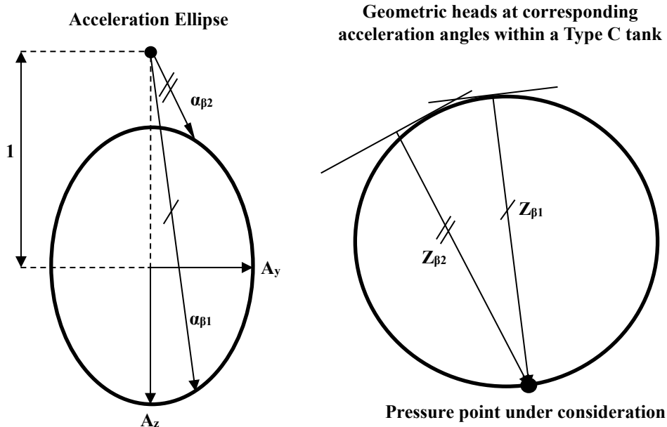
CR Fig. 4-3 Maximum Dynamic Pressure Differential
