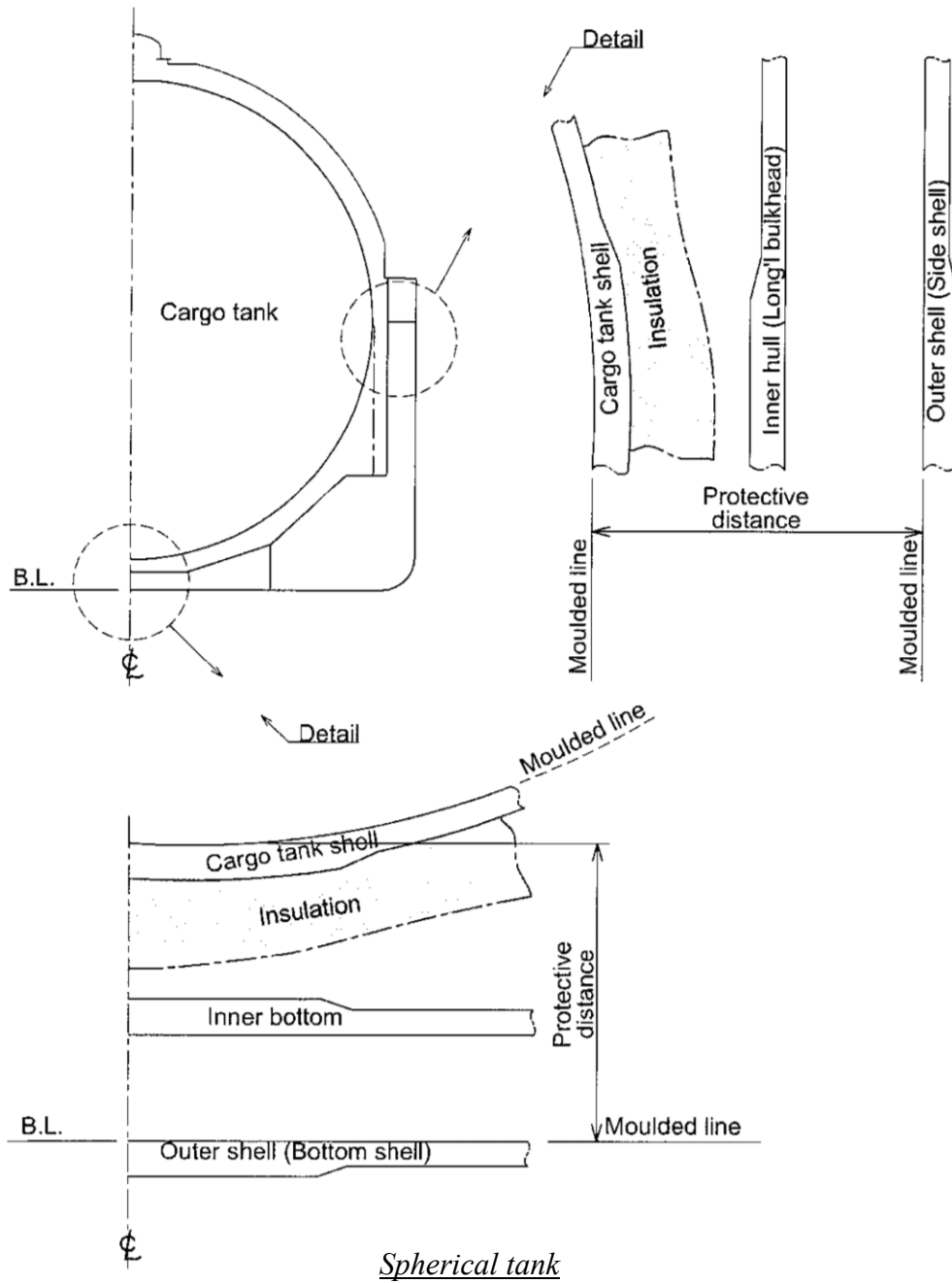
Figure 2.5(d) – Protective Distance
