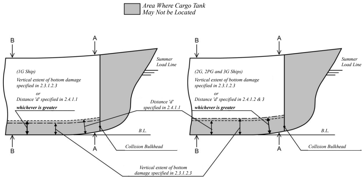
Centreline Profile - Type 1G, 2G, 2PG and 3G ships
