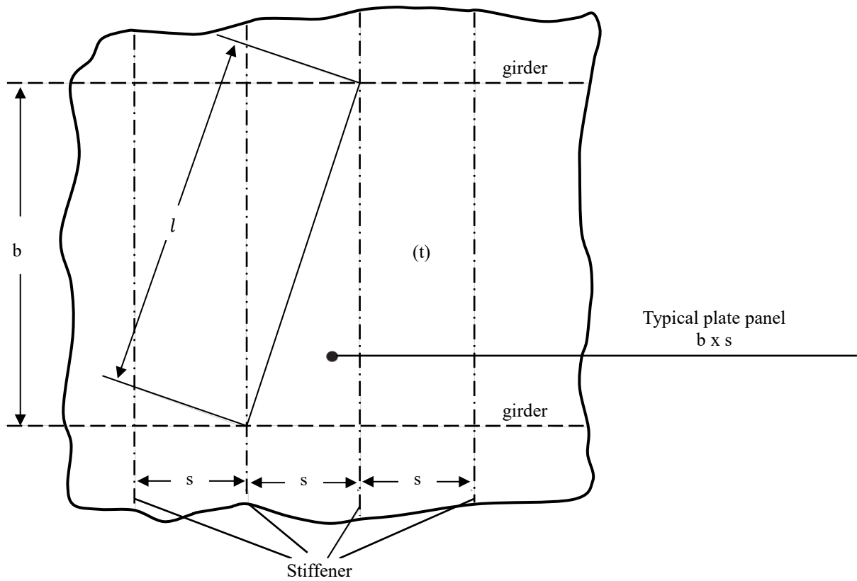
CR Fig. 8-1 Design Crack
