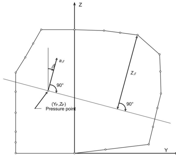
Figure 4.2 - Determination of Internal Pressure Heads
