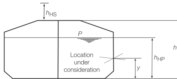
CR Fig. 4-2 Test Head(s)
