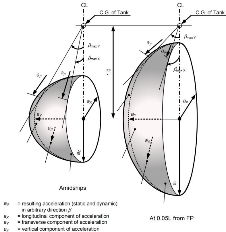
Figure 4.1 - Acceleration ellipsoid
