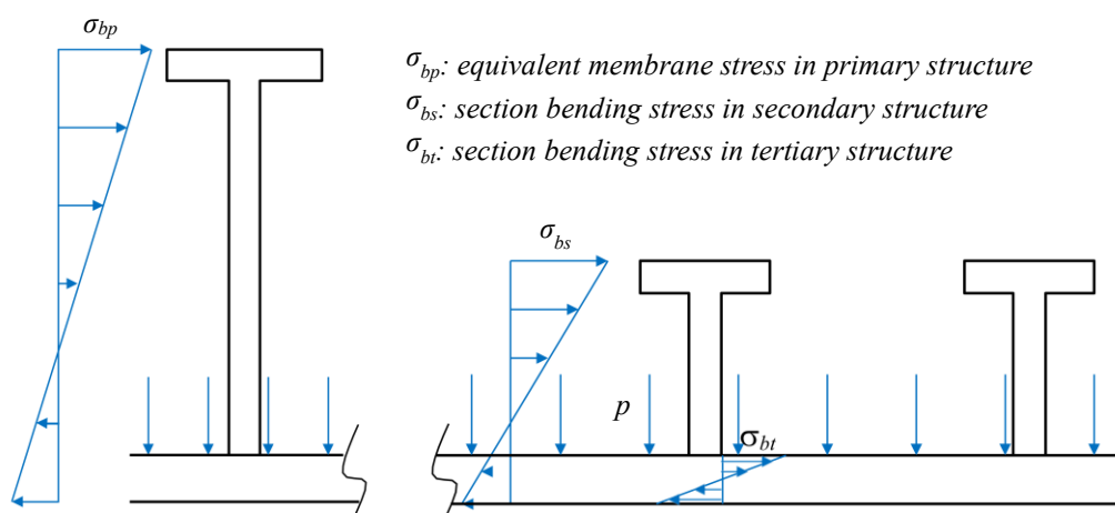
Figure 1: Definition of the three categories of section stress (Stress \sigma_{bp} and \sigma_{bs} are normal to the cross section shown.)
