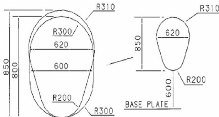
CR Fig. 3-2 Alternative Vertical Openings
