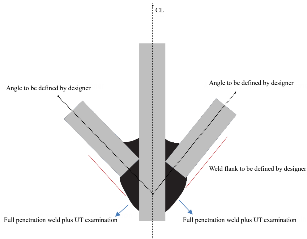
CR Fig. 4-1 Cruciform Full Penetration Weld
