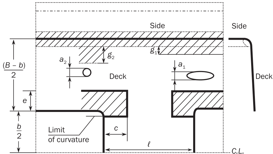
Figure 15 : Position of openings in strength deck
