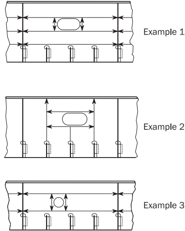
Figure 13 : Web plate with openings
