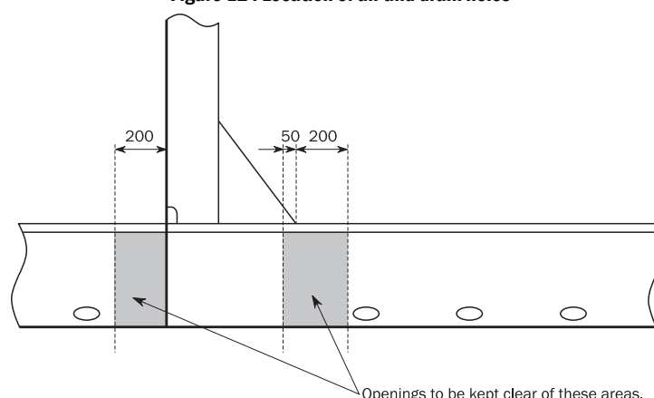
Figure 12 : Location of air and drain holes
