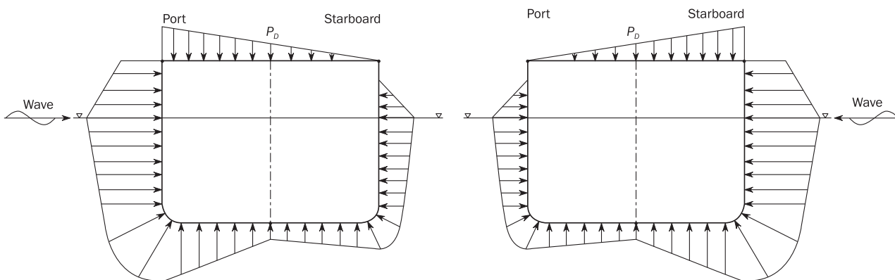
Figure 7 : Transverse distribution of dynamic pressure for BSP-2P (left) and BSP-2S (right) load cases
