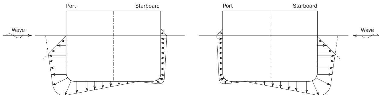
Figure 9 : Transverse distribution of dynamic pressure amidships for OST-2P (left) and OST-2S (right) load cases
