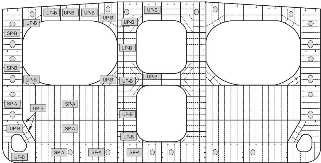
Figure 4 : Cross tie
