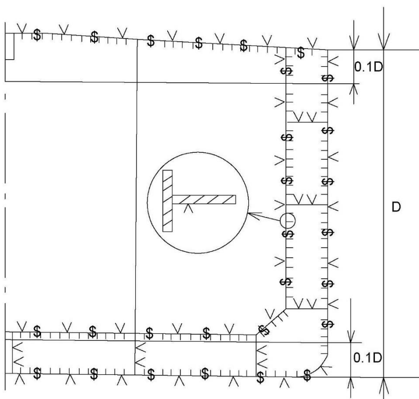
Figure 5: Transverse section
