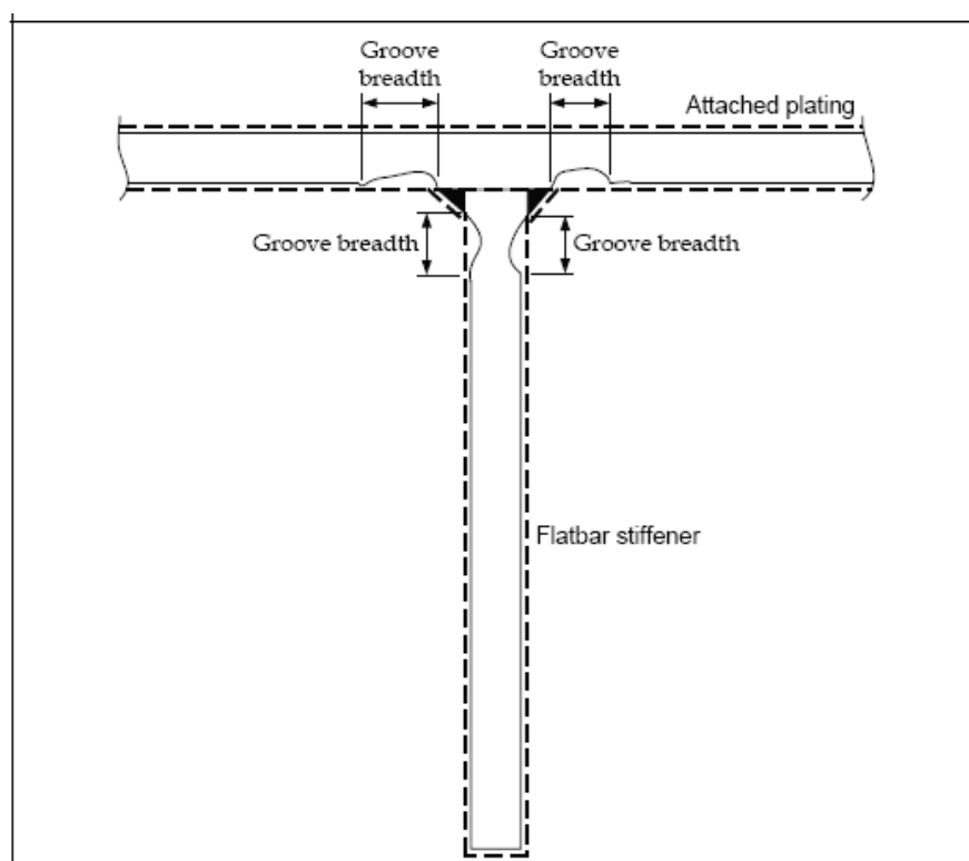
Figure 3: Grooving corrosion
