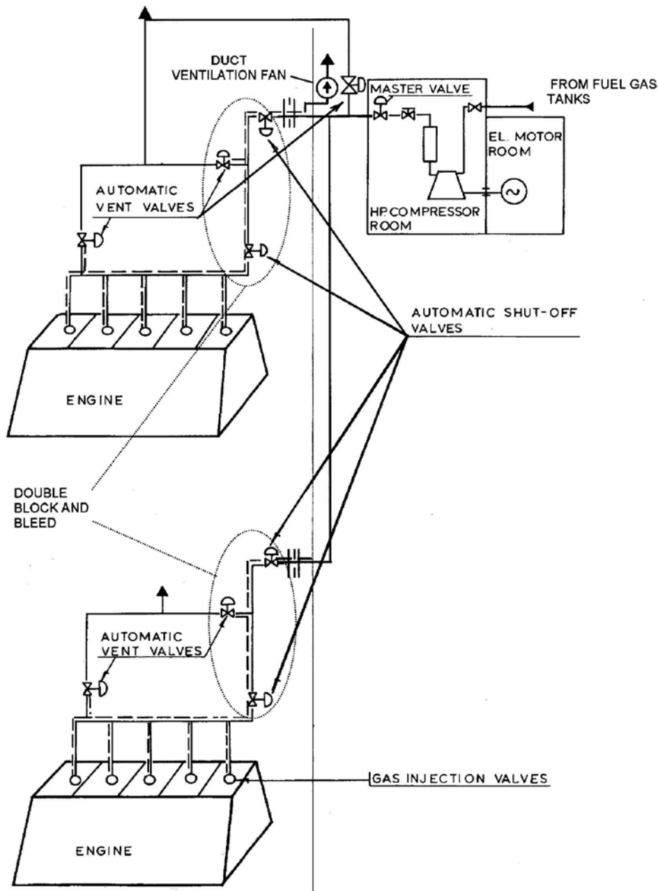
Figure 5-2 Alternative supply valve arrangements for high-pressure installations (multi-engine installation)
